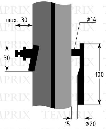
Detail X
